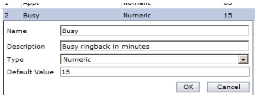
Figure 88 Editing scheduling script parameter from the Scheduling Parameters tab
