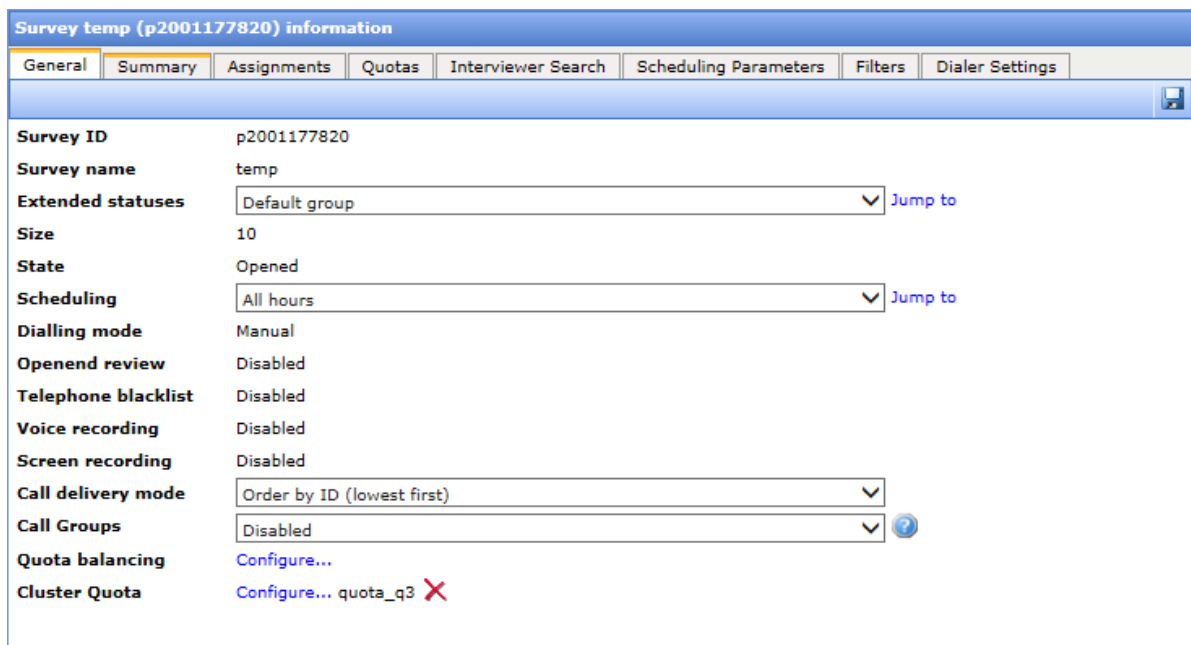
Figure 73 Quota clustering settings on the General tab in survey View mode
