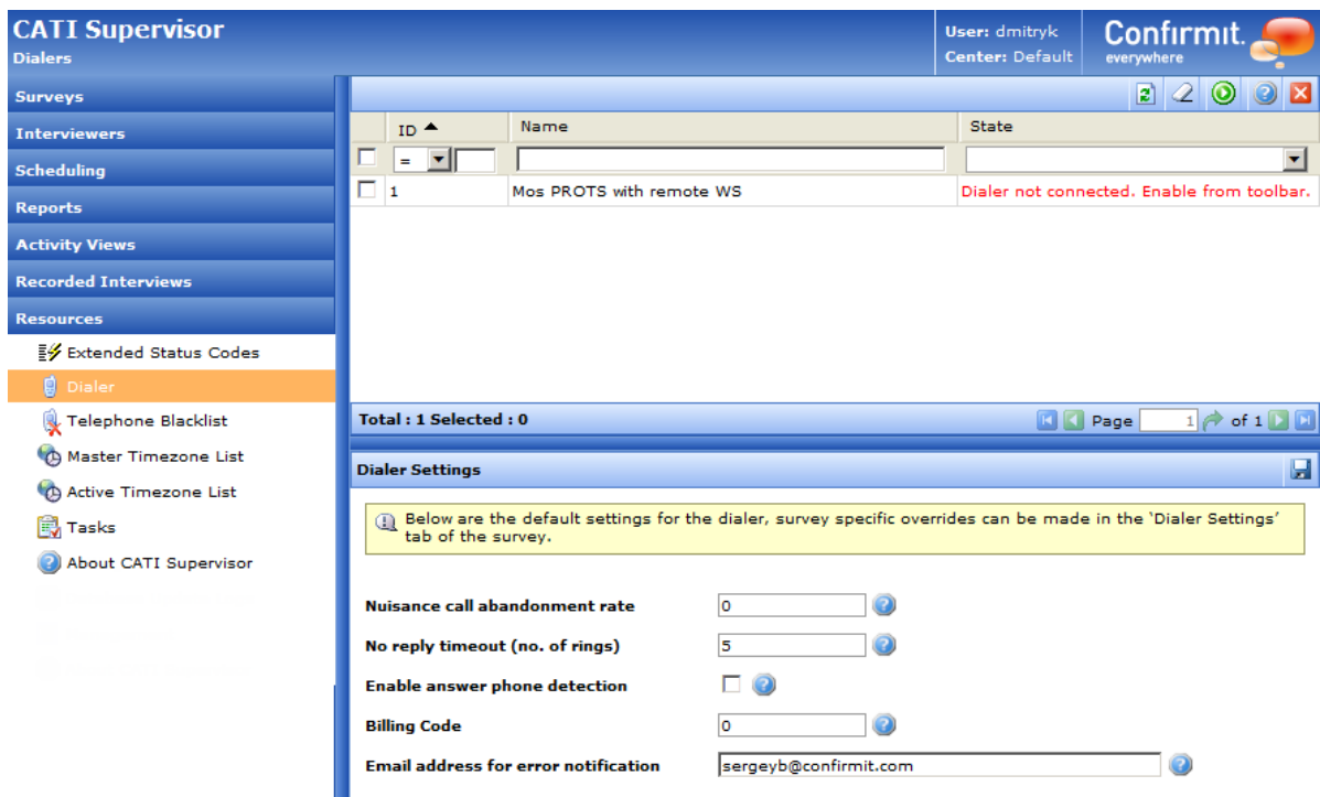
Figure 264 The Dialer object tab with the Pro-T-S type of dialers
