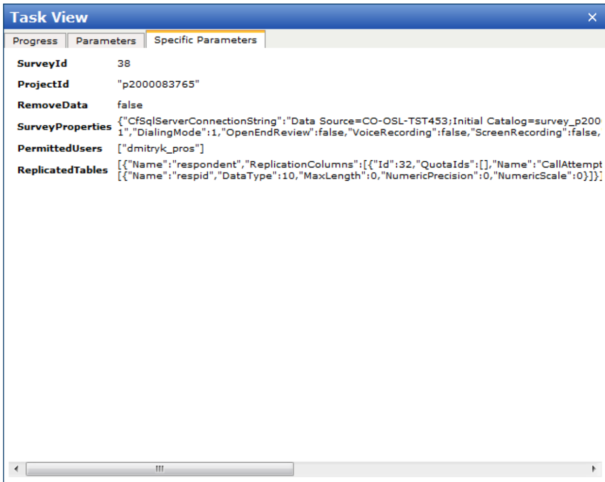
Figure 276 Task View dialog window - Specific Parameters tab
