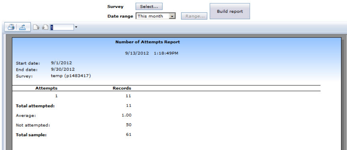
Figure 312 The generated Number of Attempts Report
