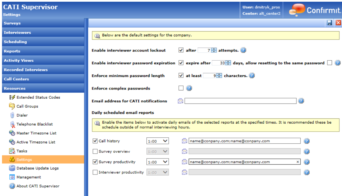
Figure 279 Configuring interviewer account locking settings
