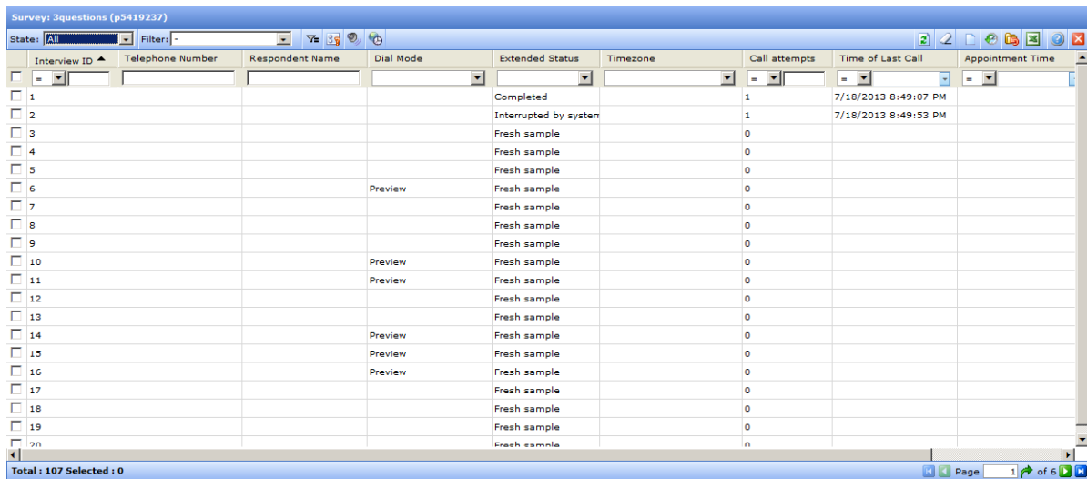
Figure 130 Choosing the dial mode in the Call Management window
