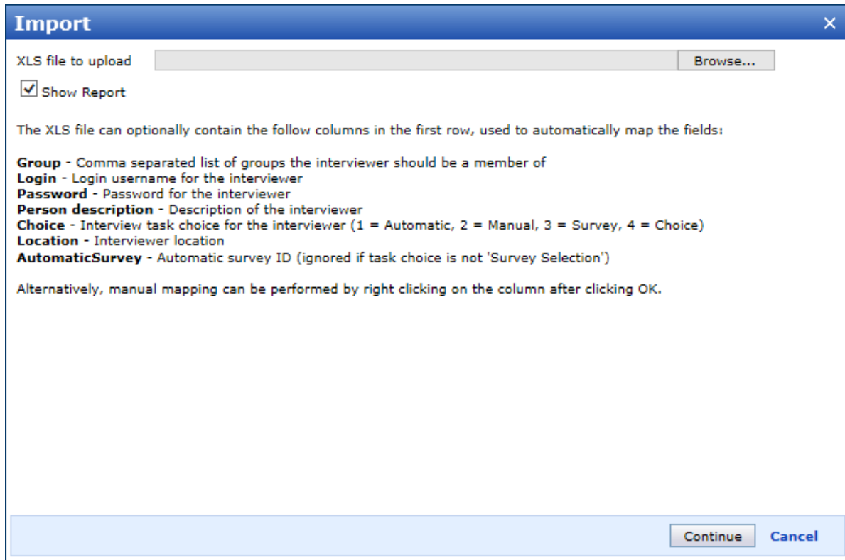
Figure 50 Importing the interviewer list from a file
