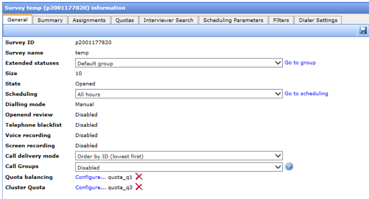
Figure 60 Survey properties displayed in the bottom right frame
