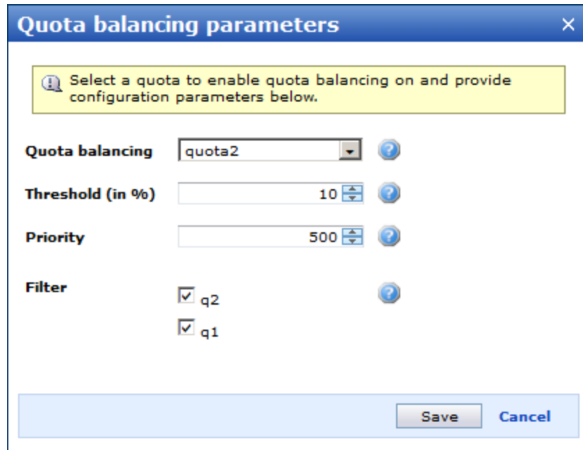
Figure 68 Specifying the Quota Balancing settings
