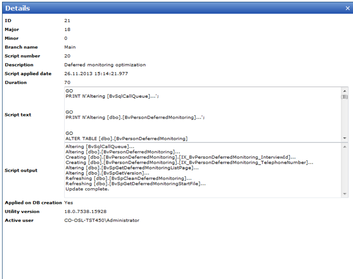
Figure 281 Checking database update details
