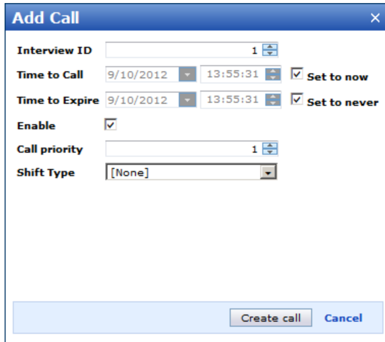
Figure 112 Adding/modifying the call properties
