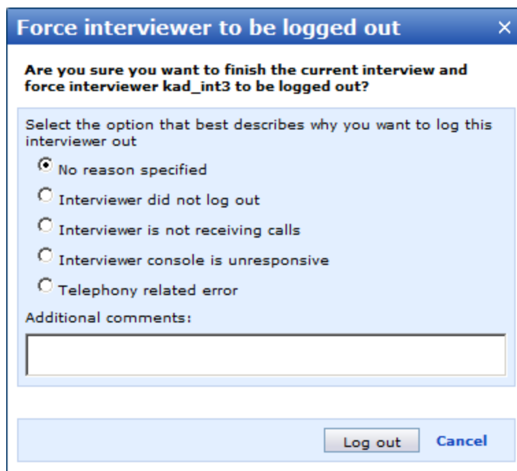
Figure 244 A dialog displayed when the supervisor tries to terminate the interview (force the logout)
